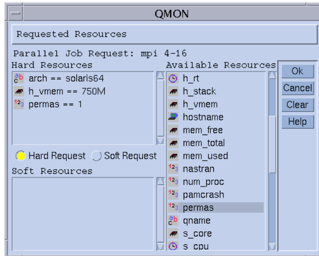
FIGURE 3-7 Requested Resources Dialog Box
