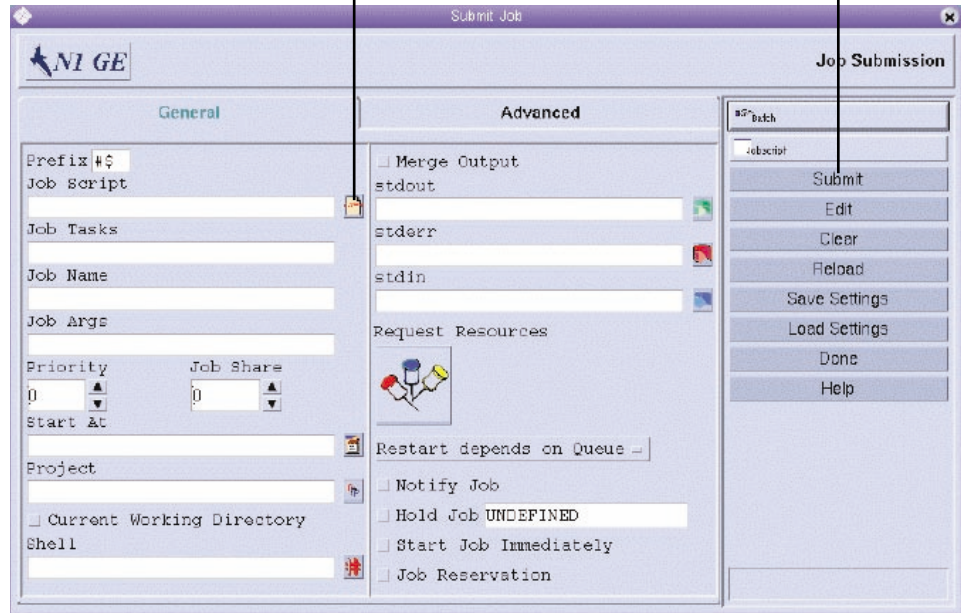
FIGURE 3-2 Submit Job Dialog Box
